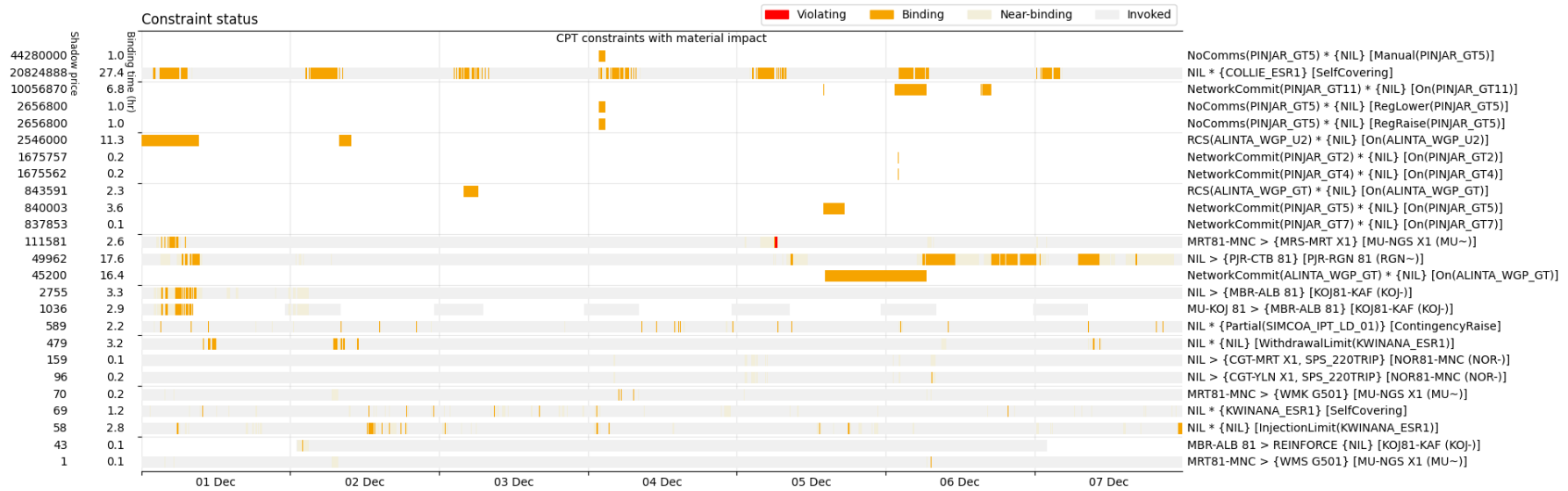
Figure 3 – Binding summary of library constraints.
