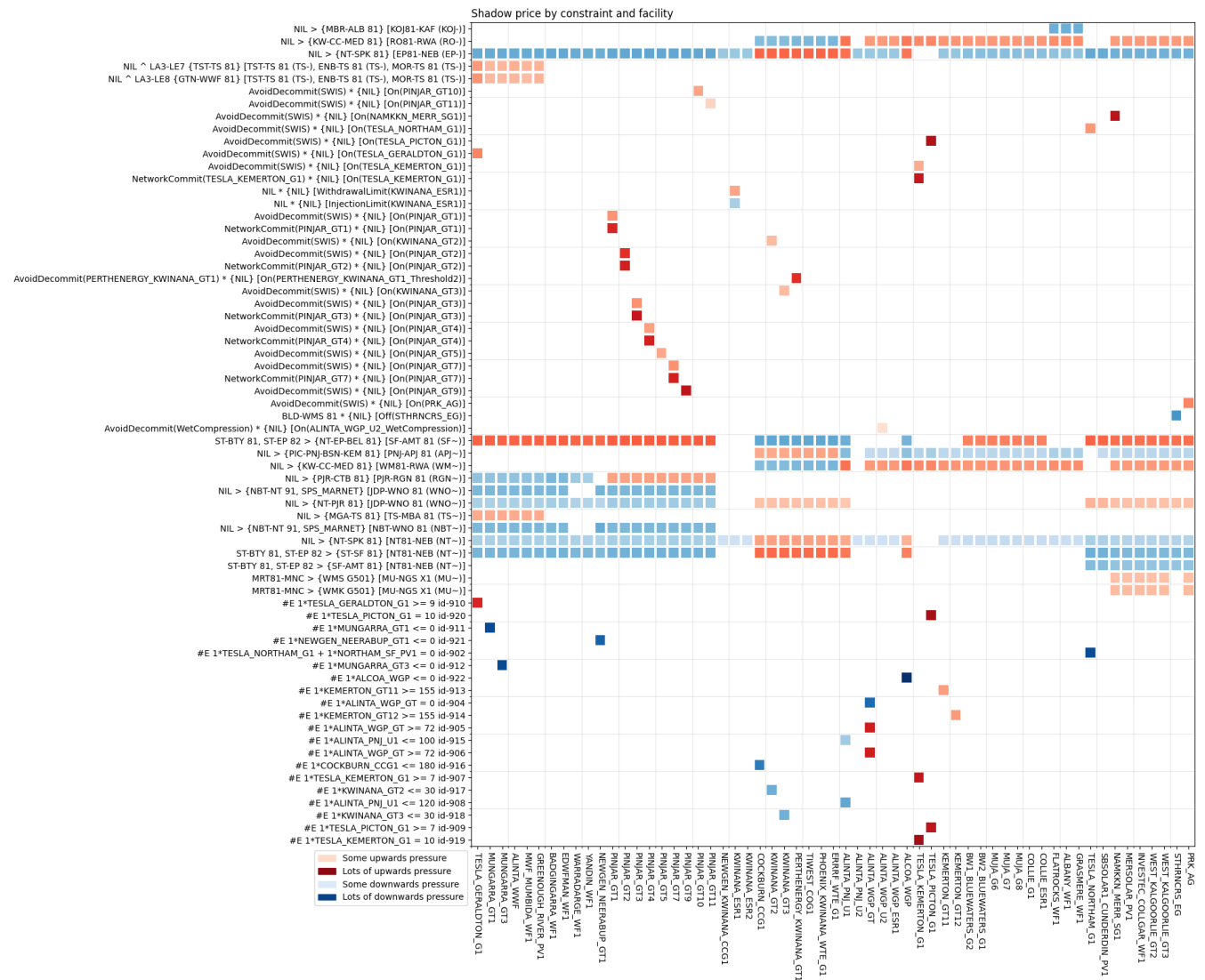
Figure 4 – Summary of shadow price by constraint and by Facility.
