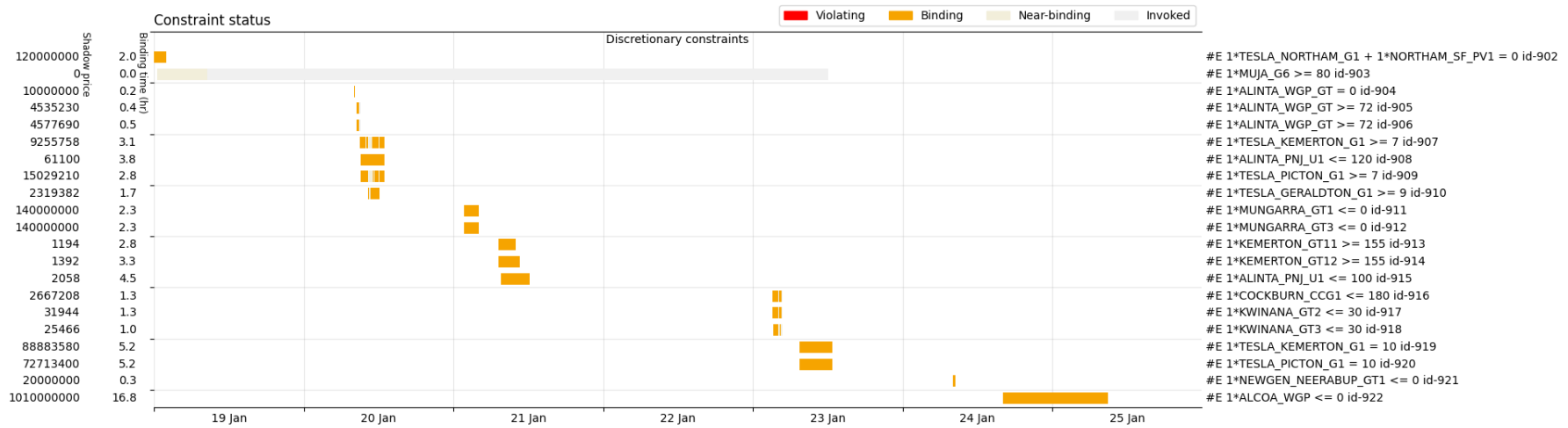
Figure 2 – Binding summary of discretionary Constraint Equations.
