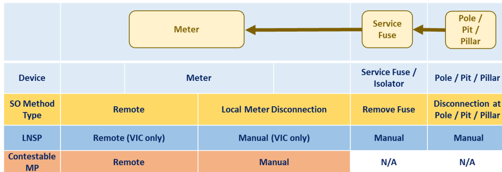
Figure 16 De-Energisation Methods
