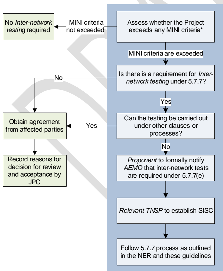
Figure 2 Assessment of whether inter-network test is required – activities 1 to 4 (see Appendix F)
