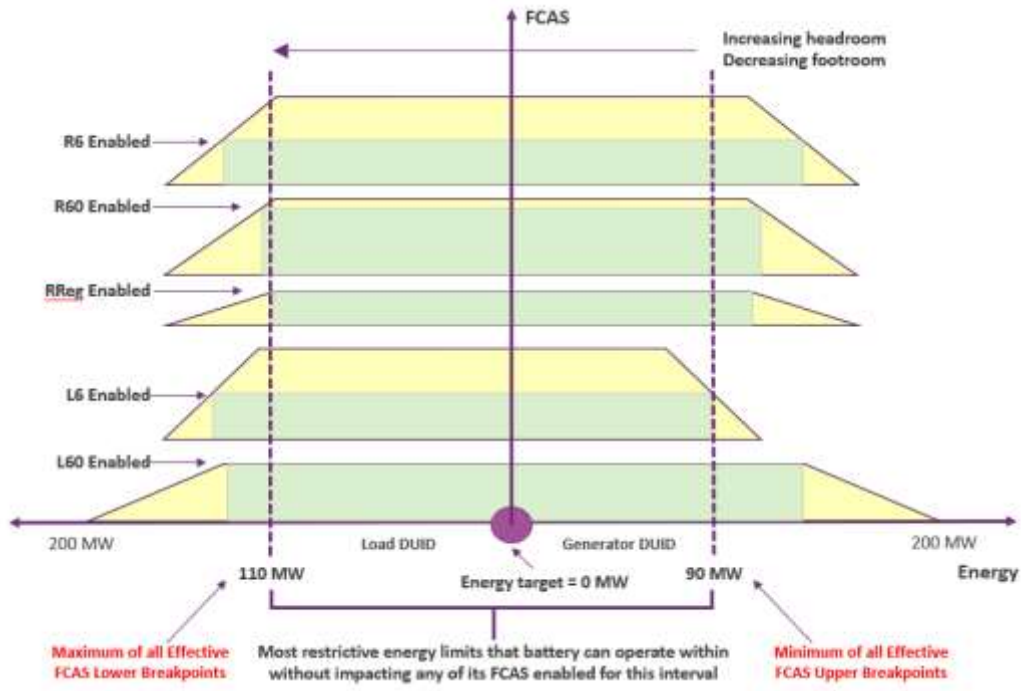
Figure 4 Operating Limits based on the most restrictive FCAS breakpoints
