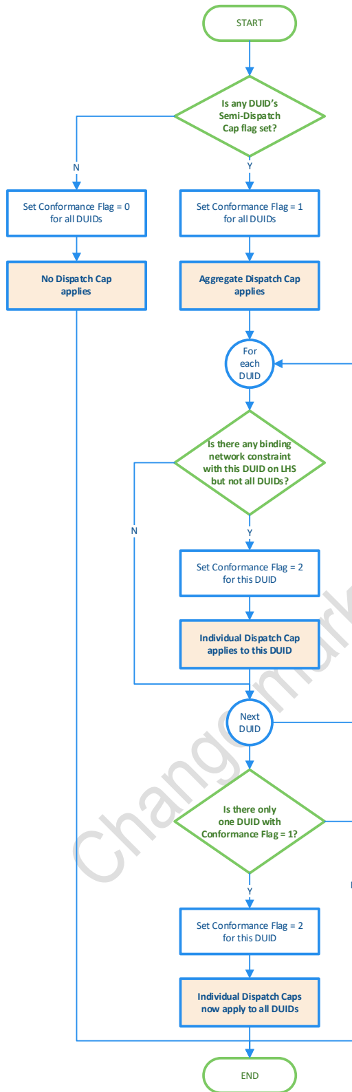
Figure 1 Dispatch conformance logic for a Cap Aggregate
