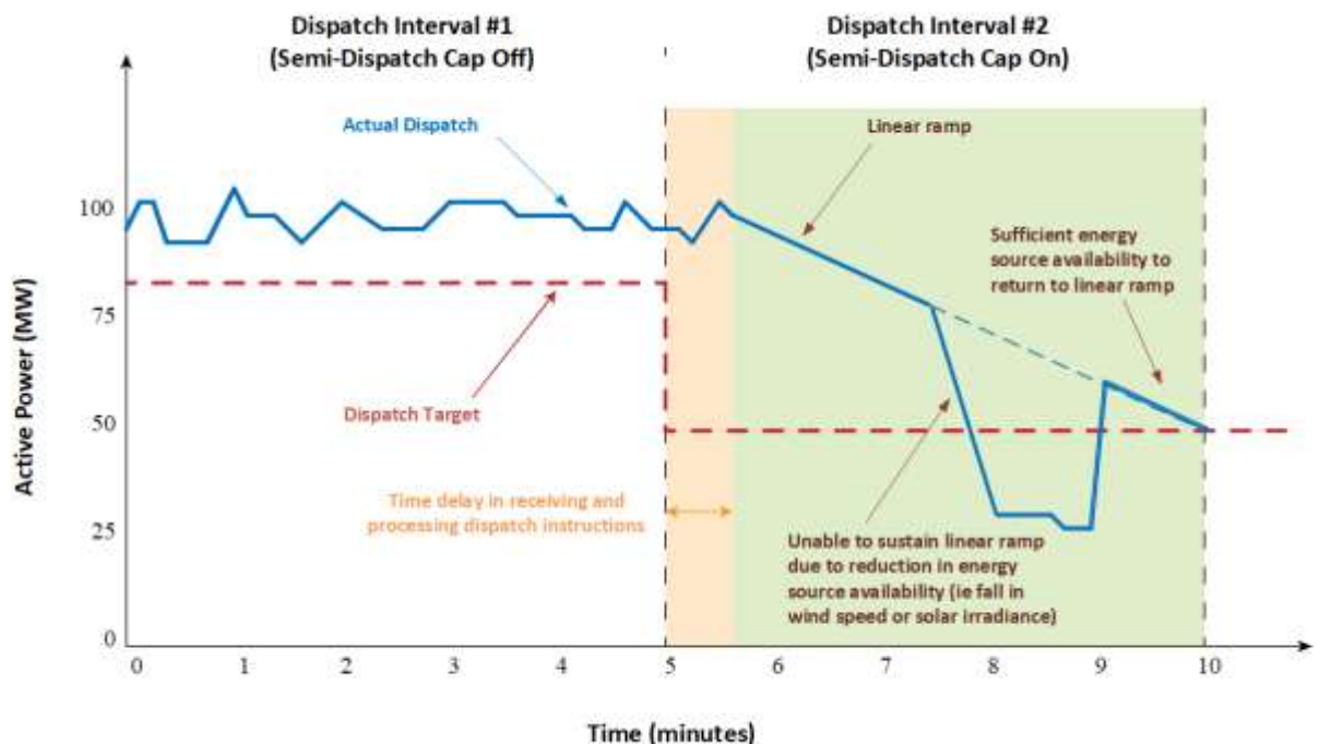
Figure 6 Semi-scheduled generating unit cannot sustain linear ramp due to reduction in energy available
