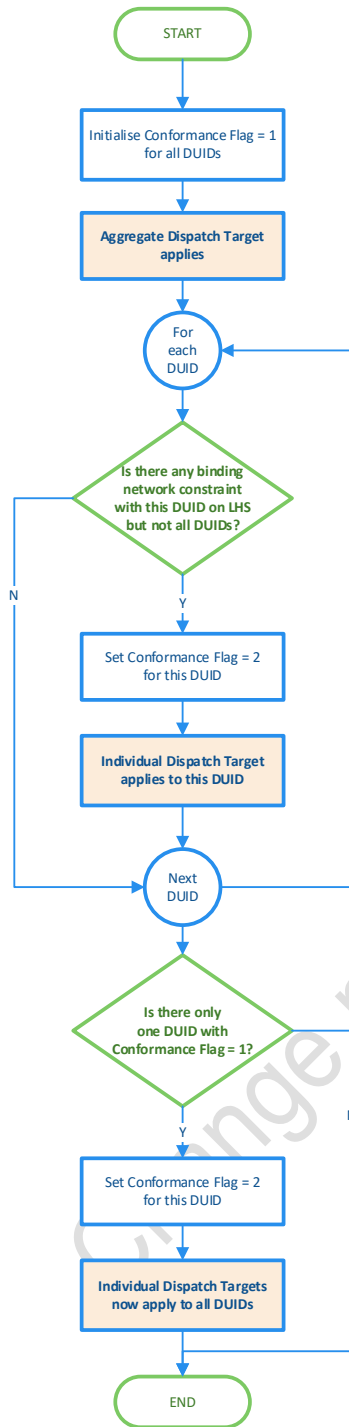
Figure 2 Dispatch conformance logic for a Target Aggregate
