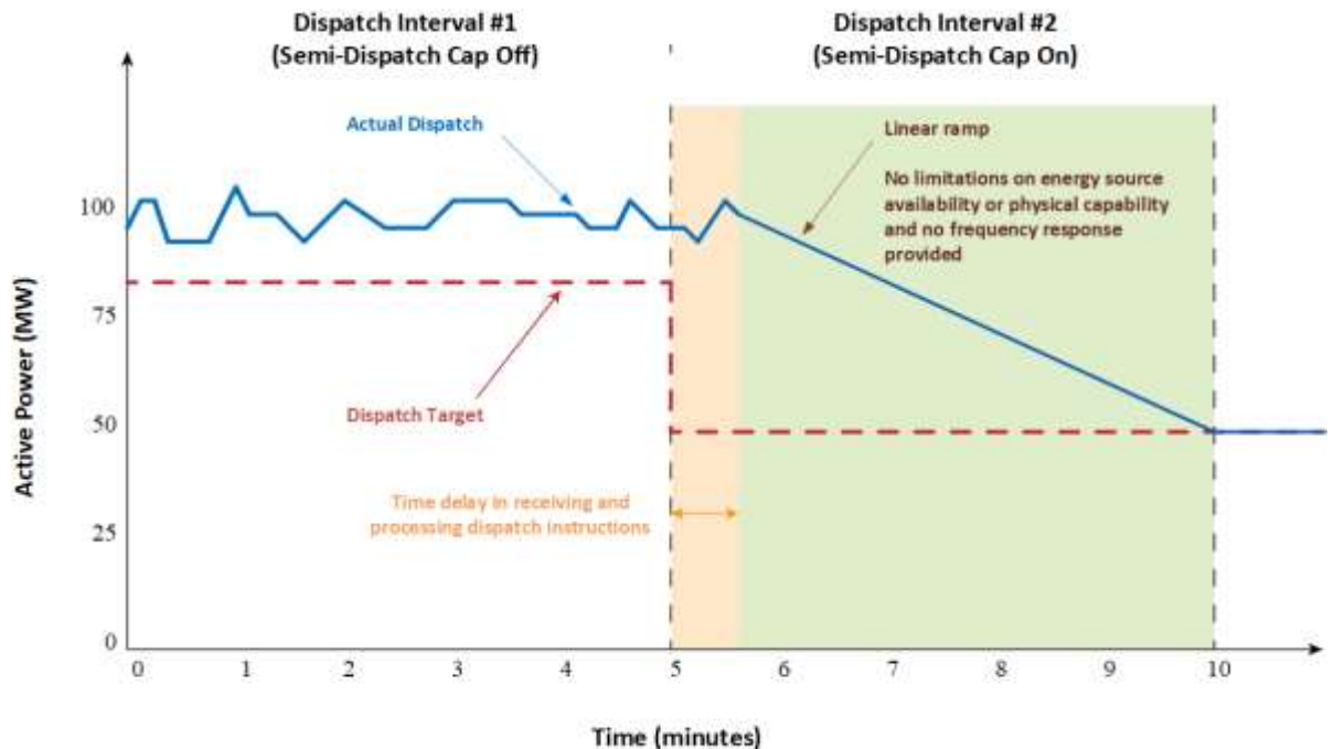
Figure 5 Semi-scheduled generating unit linear ramping with no limiting factors
