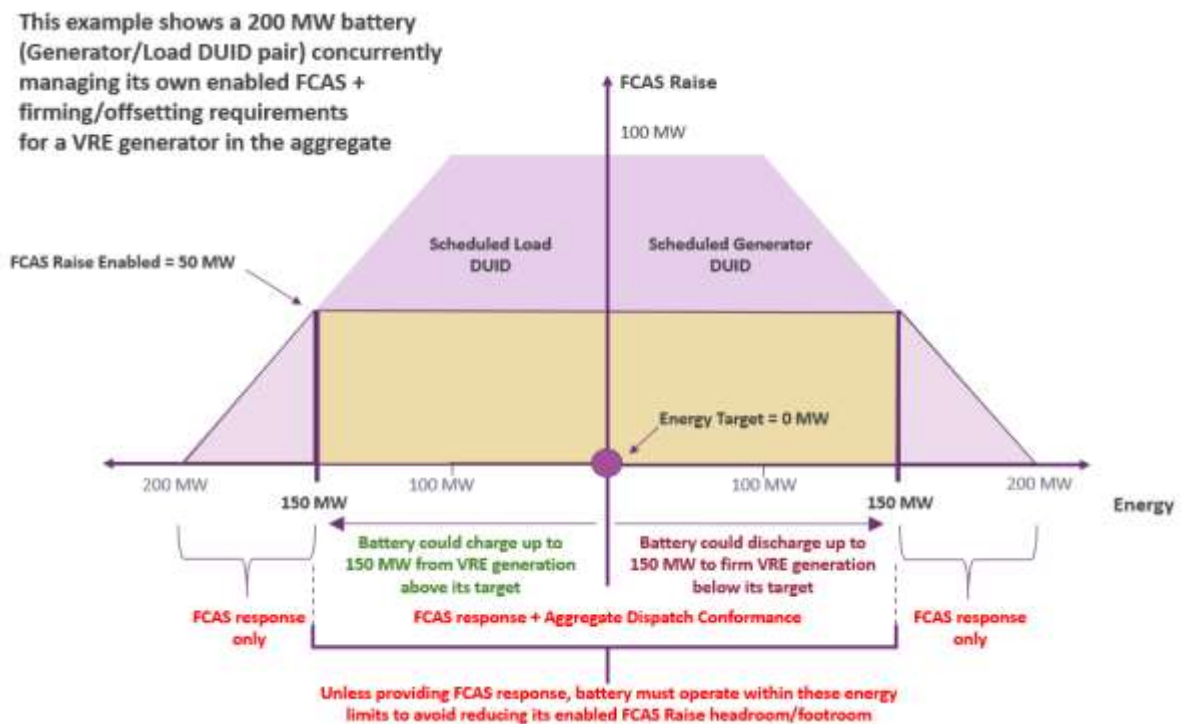
Figure 3 Operating Limits for managing FCAS and Aggregated Dispatch in a Target Aggregate
