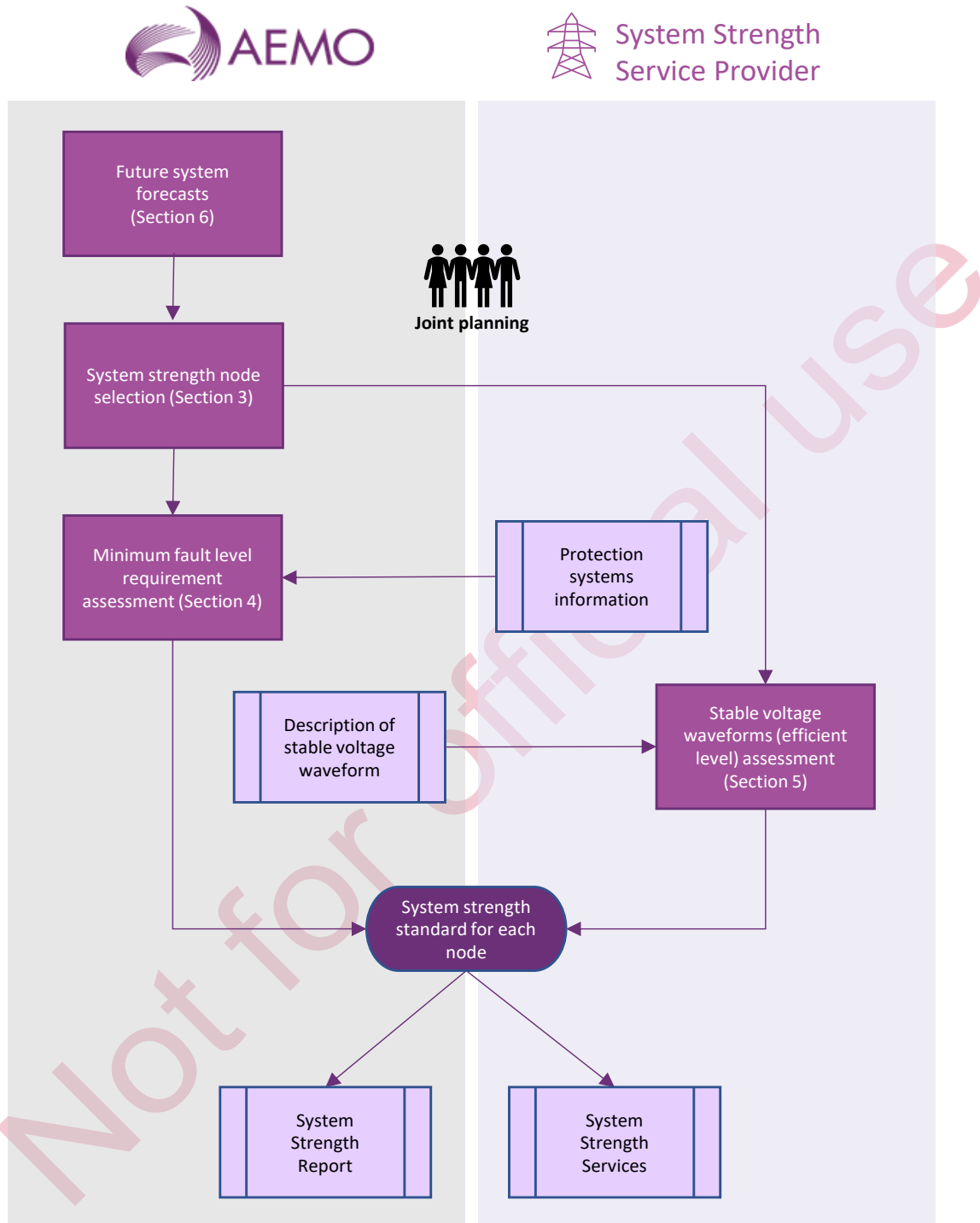
Figure 1 System Strength Requirements Methodology overview
