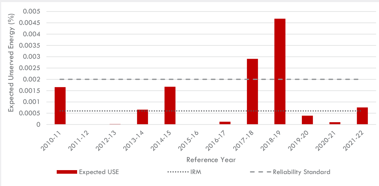
Figure 3 Figure 4 Unserviced energy by Reference Year
