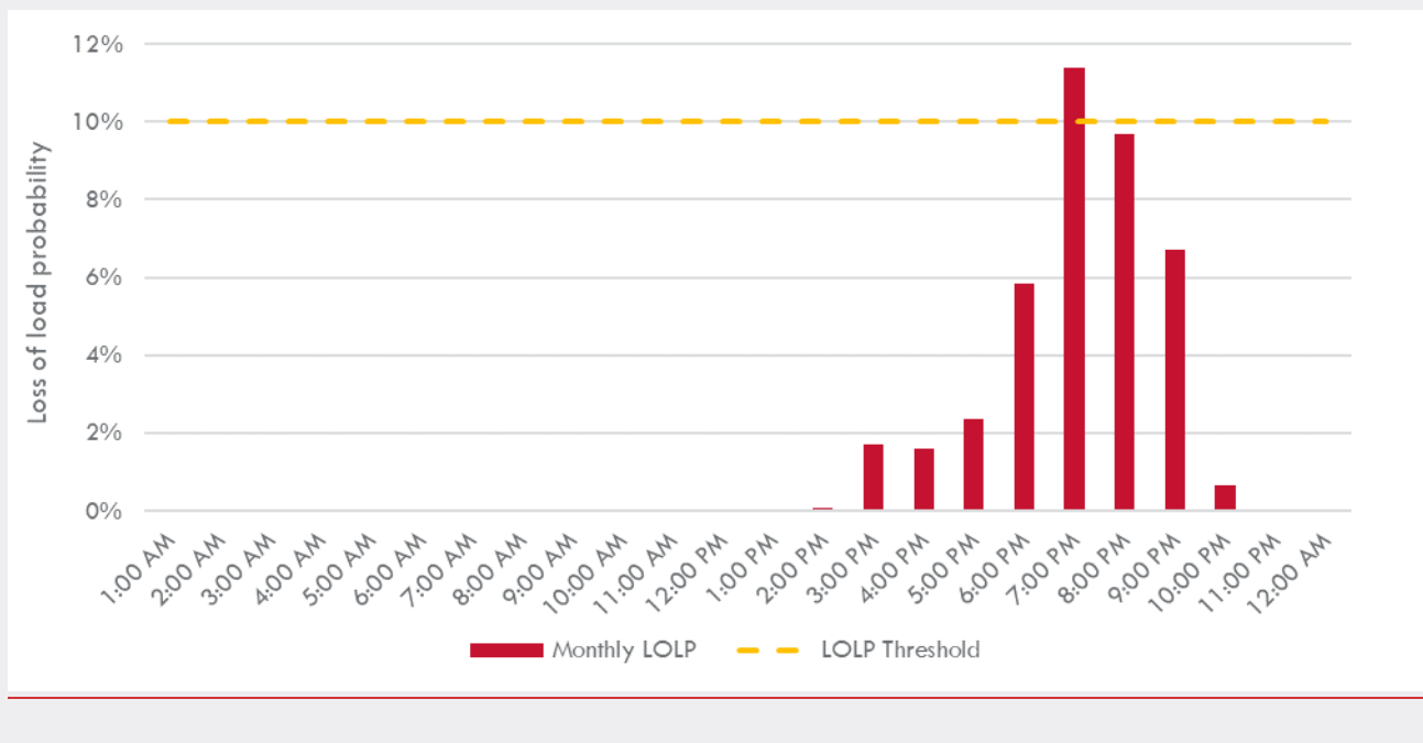
Figure 7 Time of day probability of lost load assessment (all identified months)
